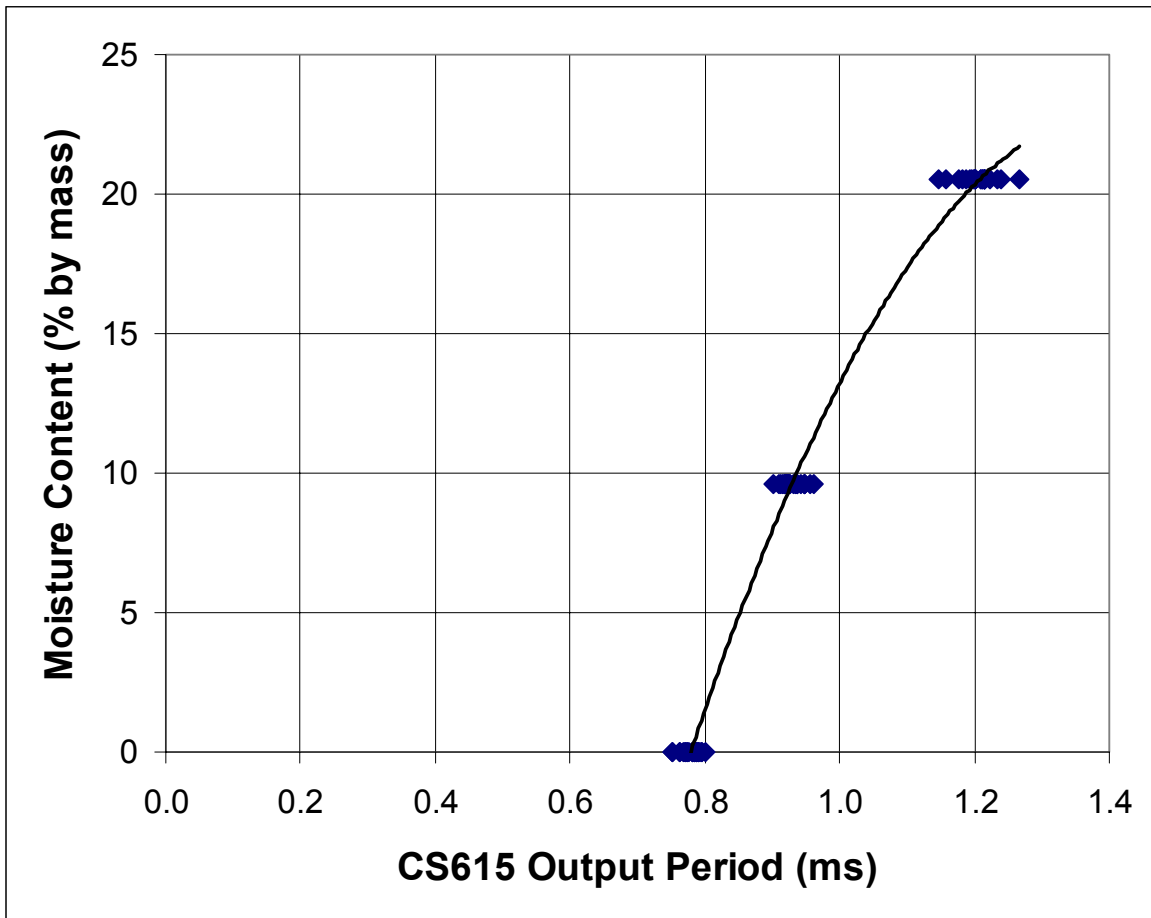
Figure 5. Calibration data and best-fit composite curve for CS615 moisture probes
