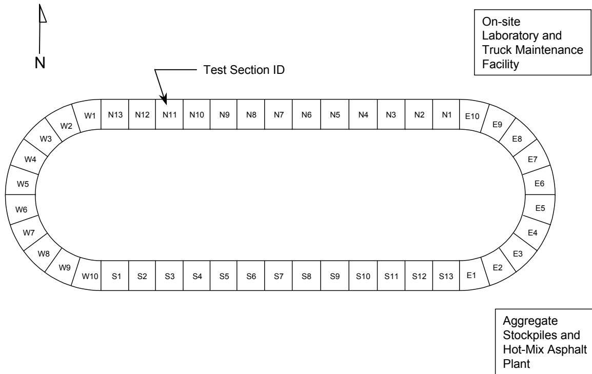
Figure 1. Track layout
