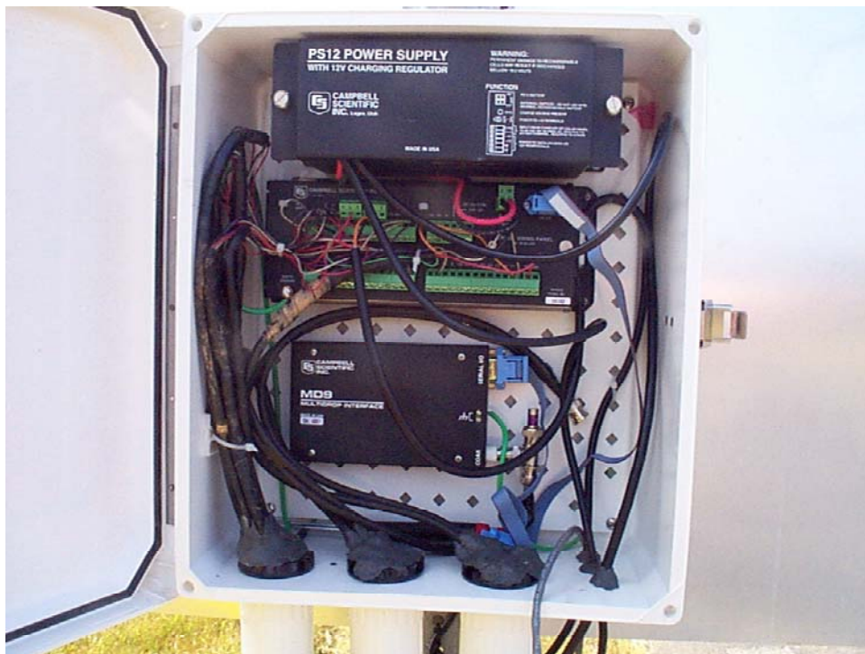
Photo 6. View inside the Campbell Scientific enclosure
