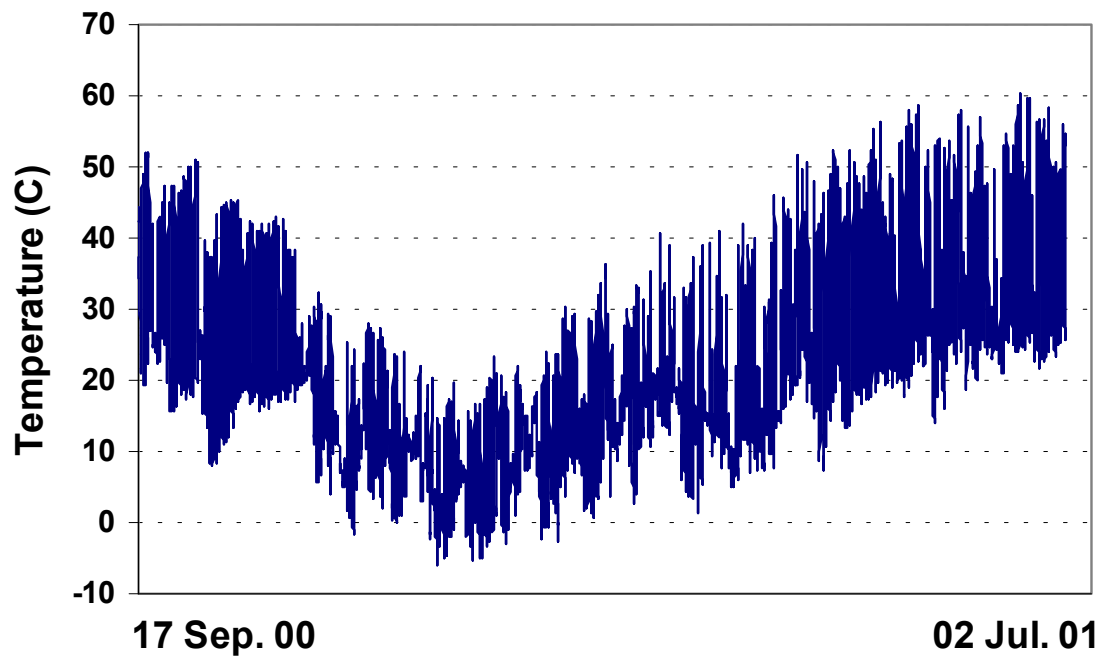
Figure 12. Temperature at pavement surface for test section S1 [ F = 9/5(C) + 32 ]
