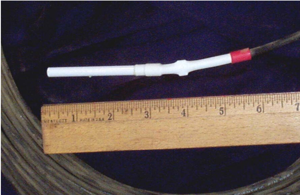
Photo 3. Temperature probe, Campbell Scientific Model 108
