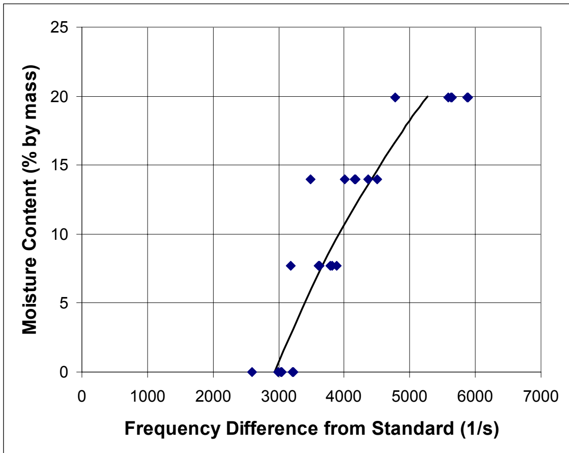
Figure 6. Calibration data and best-fit composite curve for Troxler moisture probes
